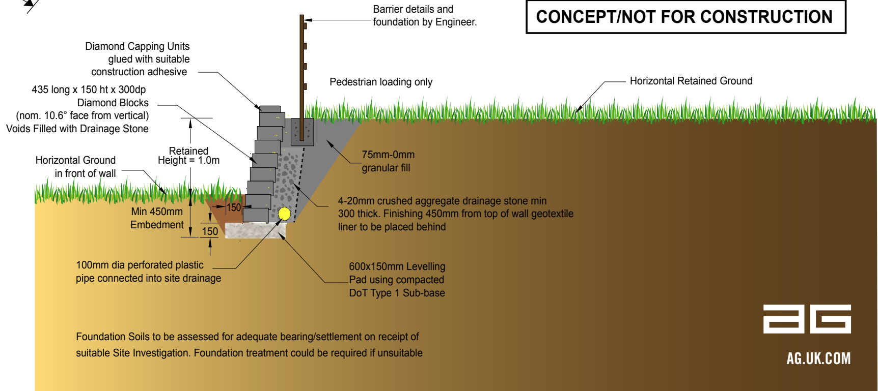
TYPICAL SECTION FOR A 1.0m RETAINED HEIGHT DIAMOND WALL
