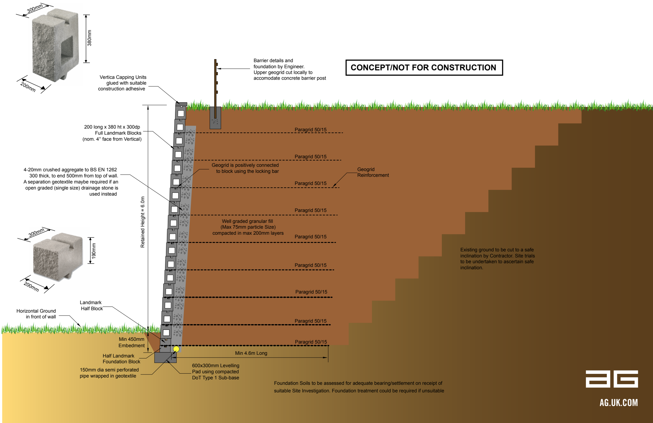
TYPICAL SECTION FOR A 6.0m RETAINED HEIGHT LANDMARK WALL
